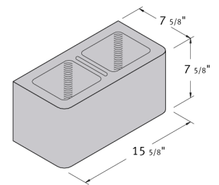
8 x 8 x 16 Double Bullnose Face
