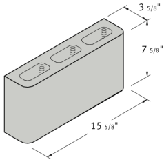
4 x 8 x 16 Double Bullnose Face
