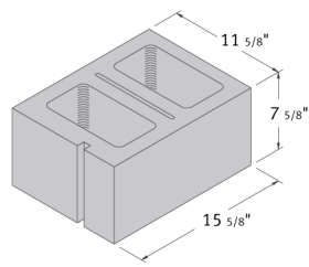
12 x 8 x 16 Sash
