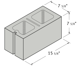
8 x 8 x 16 Sash
