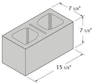
8 x 8 x 16 2 Hour Rated
