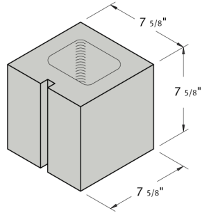
8 x 8 x 8 Half
