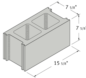
8 x 8 x 16 Regular
