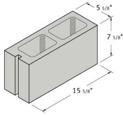
6 x 8 x 16 Regular
