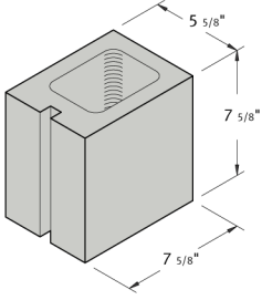
6 x 8 x 8 Half
