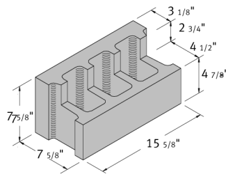
8 x 8 x 16 Header
