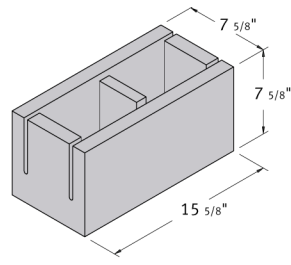
8 x 8 x 16 Knock-Out Bond Beam
