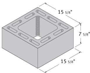
16 x 8 x 16 Pilaster
