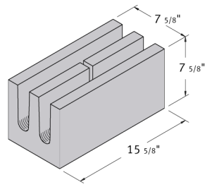
8 x 8 x 16 Solid-Bottom Bond Beam
