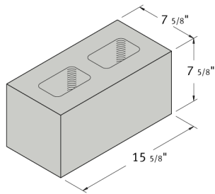
8 x 8 x 16 4 Hour Rated
