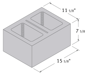
12 x 8 x 16 Regular
