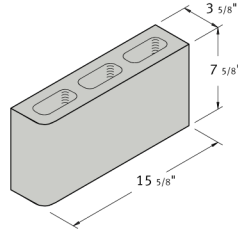
4 x 8 x 16 Single Bullnose
