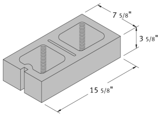
8 x 4 x 16 Half High
