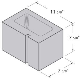
12 x 8 x 8 Half
