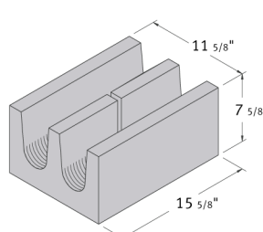
12 x 8 x 16 Solid-Bottom Bond Beam
