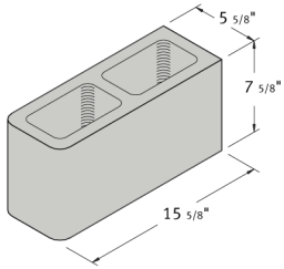
6 x 8 x 16 Double Bullnose End
