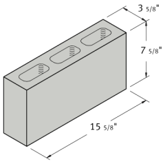
4 x 8 x 16 Partition
