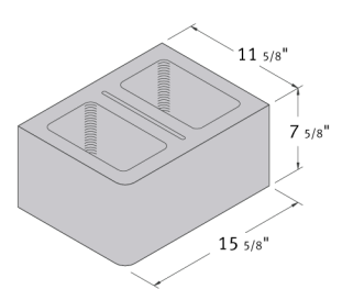
12 x 8 x 16 Single Bullnose
