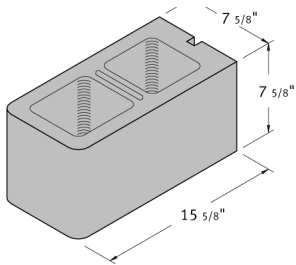
8 x 8 x 16 Double Bullnose End
