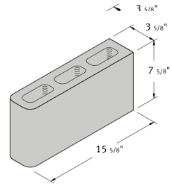
4 x 8 x 16 Double Bullnose End
