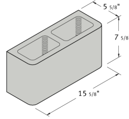
6 x 8 x 16 Double Bullnose Face
